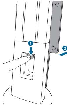
Removing the MiniPC Kit
